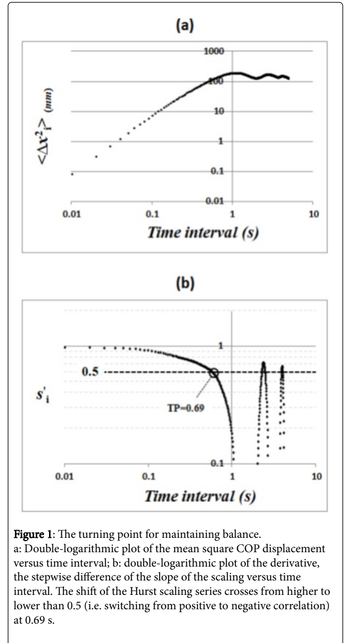
Figure 1: The turning point for maintaining balance. a: Double-logarithmic plot of the mean square COP displacement versus time interval; b: double-logarithmic plot of the derivative, the stepwise difference of the slope of the scaling versus time interval. The shift of the Hurst scaling series crosses from higher to lower than 0.5 (i.e. switching from positive to negative correlation) at 0.69 s.
